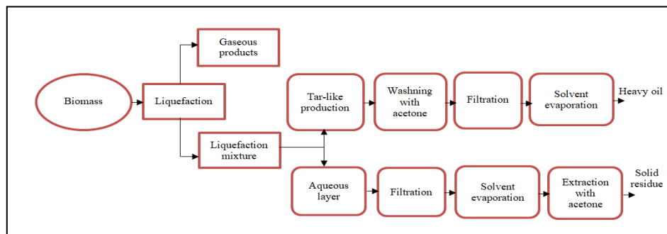
Fig. 14. Liquefaction process
