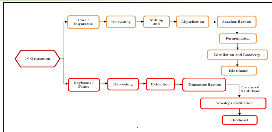
Fig. 9. First-generation biofuel processing
