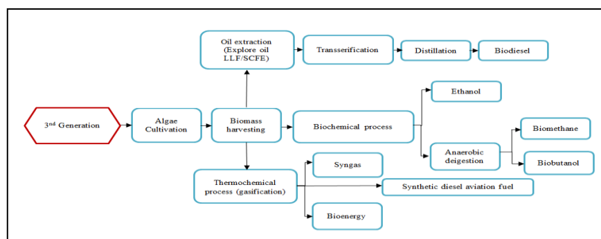
Fig. 11. Third-generation biofuel processing
