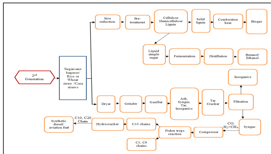
Fig. 10. Second-generation biofuel processing
