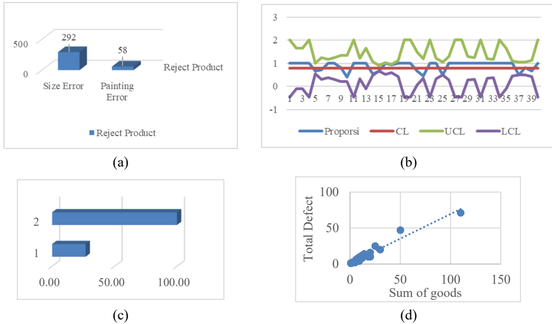
Fig. 1. The result of using quality control tools (a) Type of reject (b) P-Chart (c) Percentage of rejected goods (d) Scatterplot
